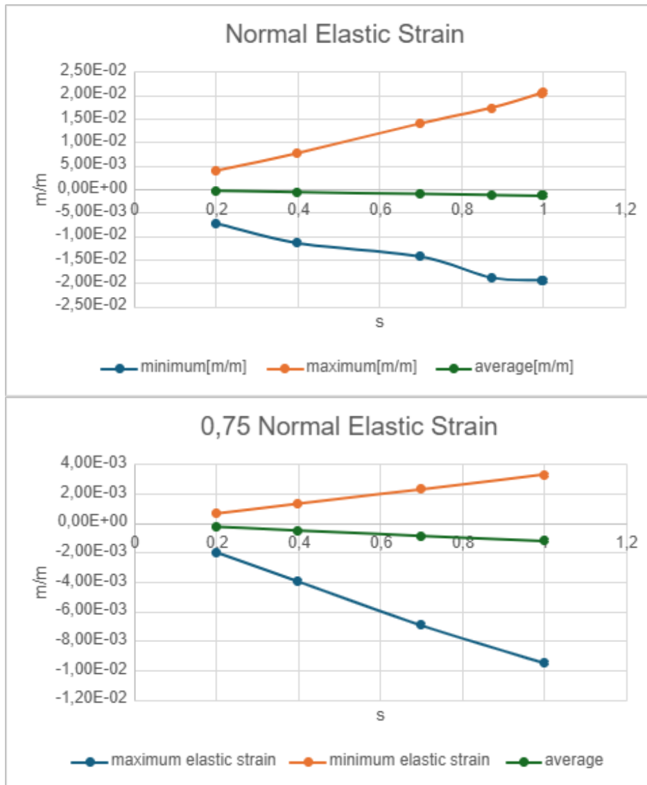
Figure 10. Normal elastic strain comparison table.
